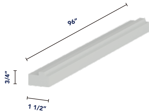
Light Rail Moulding LRM8
