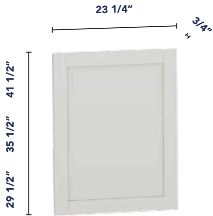
Decorative Tall Door
